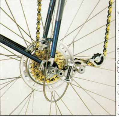
Suntour Cyclone GT Derailleur system with Suntour Tran-Z cluster and chain. Inner edges of chain's outer link plate are deeply scalloped; so chain operates at a sharper angle, engaging cluster teeth more quickly for greater shifting speed.
