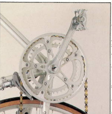
Cotterless alloy crank set for lightweight strength. Butted frame tubes also for lightweight strength. Self-balancing pedals stay in riding position.
