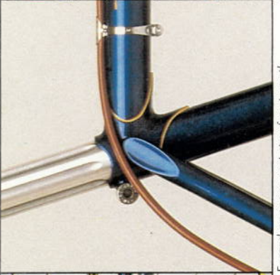
Forged concave seat stay for strength. Specially designed seat binder tube with chromoly allen head binder bolt. Laprade type fluted alloy seat post.
