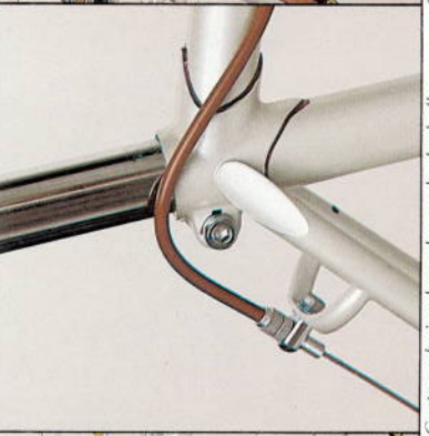
Custom design lug, chromoly dual allen head seat binder bolt for positive locking. Brazed-on rear brake cable hanger for positive adjusting, reduction of cable friction. Forged concave seat stay for strength and European good looks.
