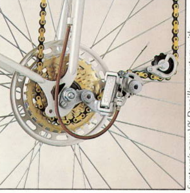
Suntour's new Vx Derailleur system with gold Train-Z chain and gold 6-speed freewheel. New cog design is as narrow as a normal 5-speed. Teeth are sharply tipped and "zigzagged" to fit each link plate precisely to enable quick, smooth speed changes.
