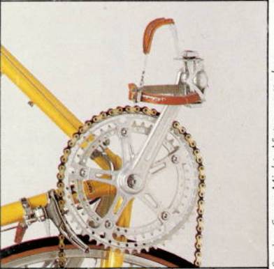
Sugino Super, Mighty Victory cotterless forged aircraft alloy crank set, for perfect chain alignment, minimum friction. Forged aluminum pedals with chromoly spindle, and precision bearing races. Toe clips, toe straps. Pro style brazed-on water bottle holder.
