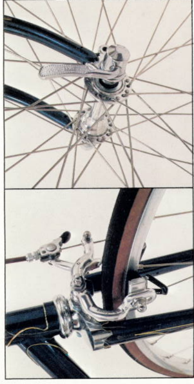
Suntour Vx small flange, quick release hubs, front and rear. Chrome forged fork end. Stainless steel spokes.
